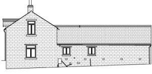
WEST ELEVATION
